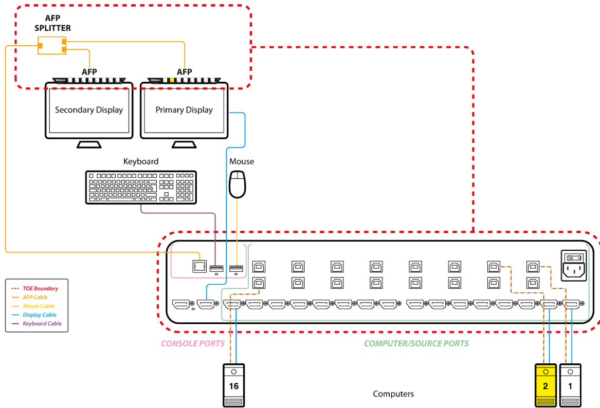
Figure 2 – KVM Multiviewer Evaluated Configuration
