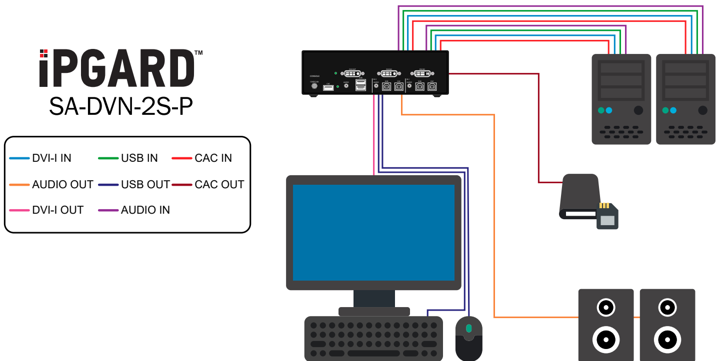
Figure 8-2: SA-DVN-2S-P
