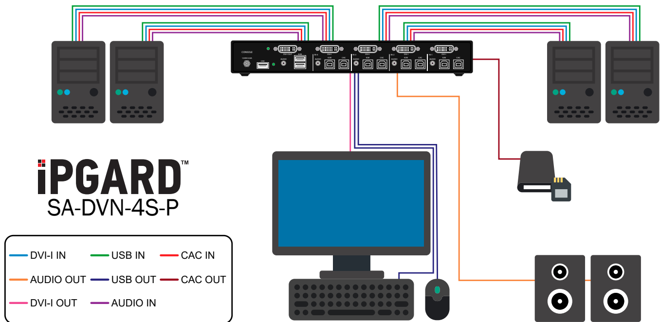
Figure 6-1: SA-DVN-4S-P
