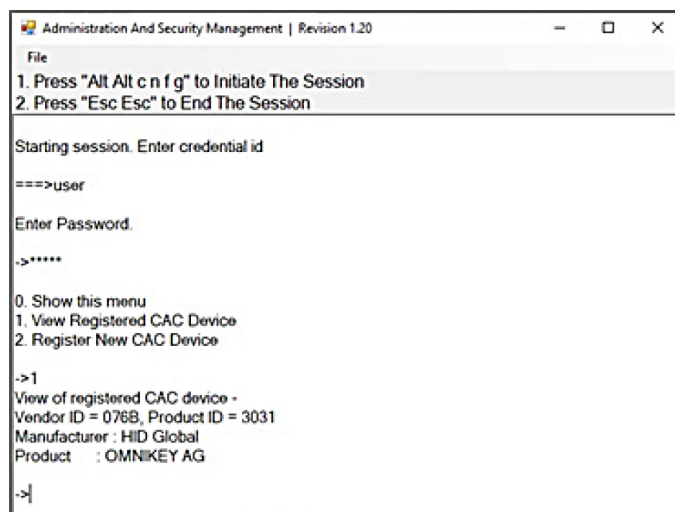
Figure 8-1 User Menu
