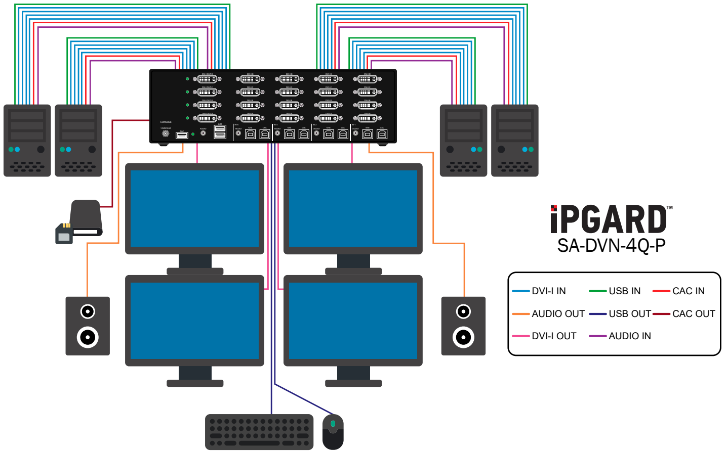
Figure 8-1: SA-DVN-4Q-P
