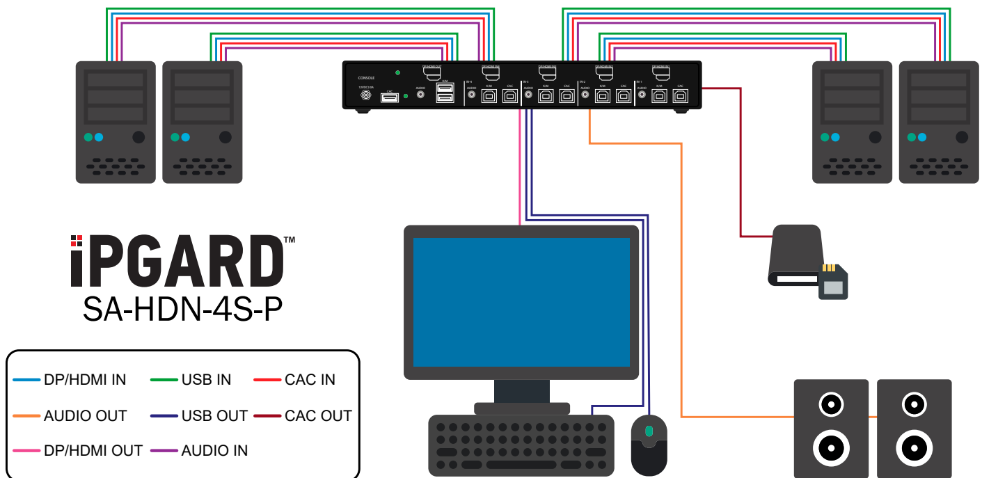
Figure 6-1: SA-HDN-4S-P
