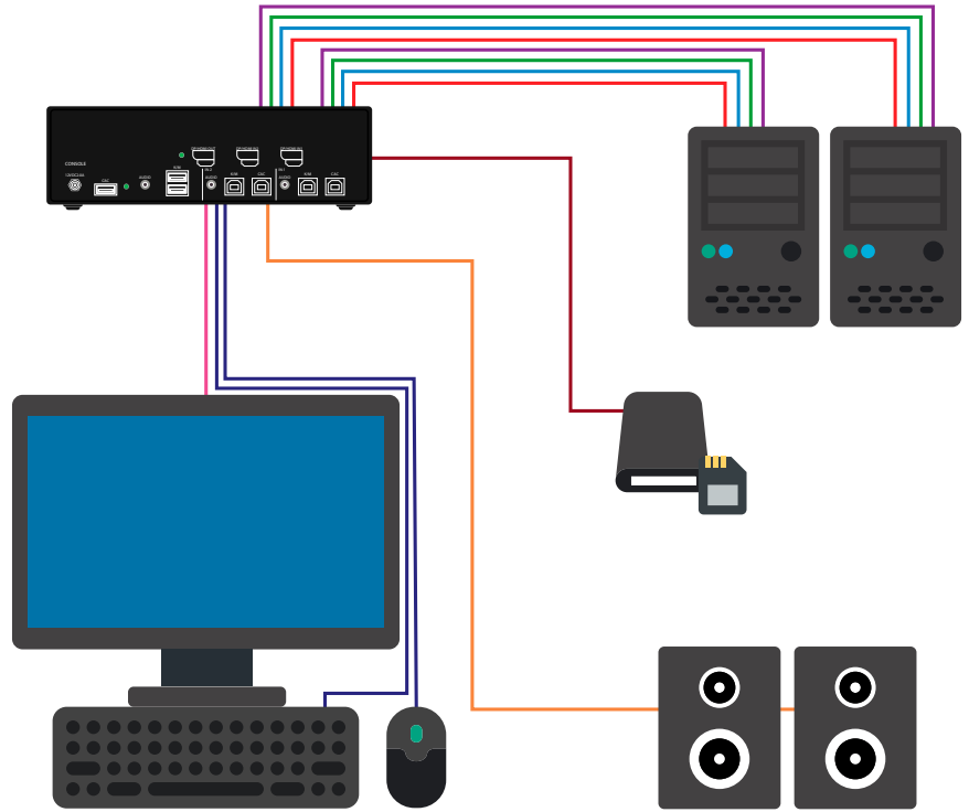
Figure 8-1: SA-HDN-2S -P
