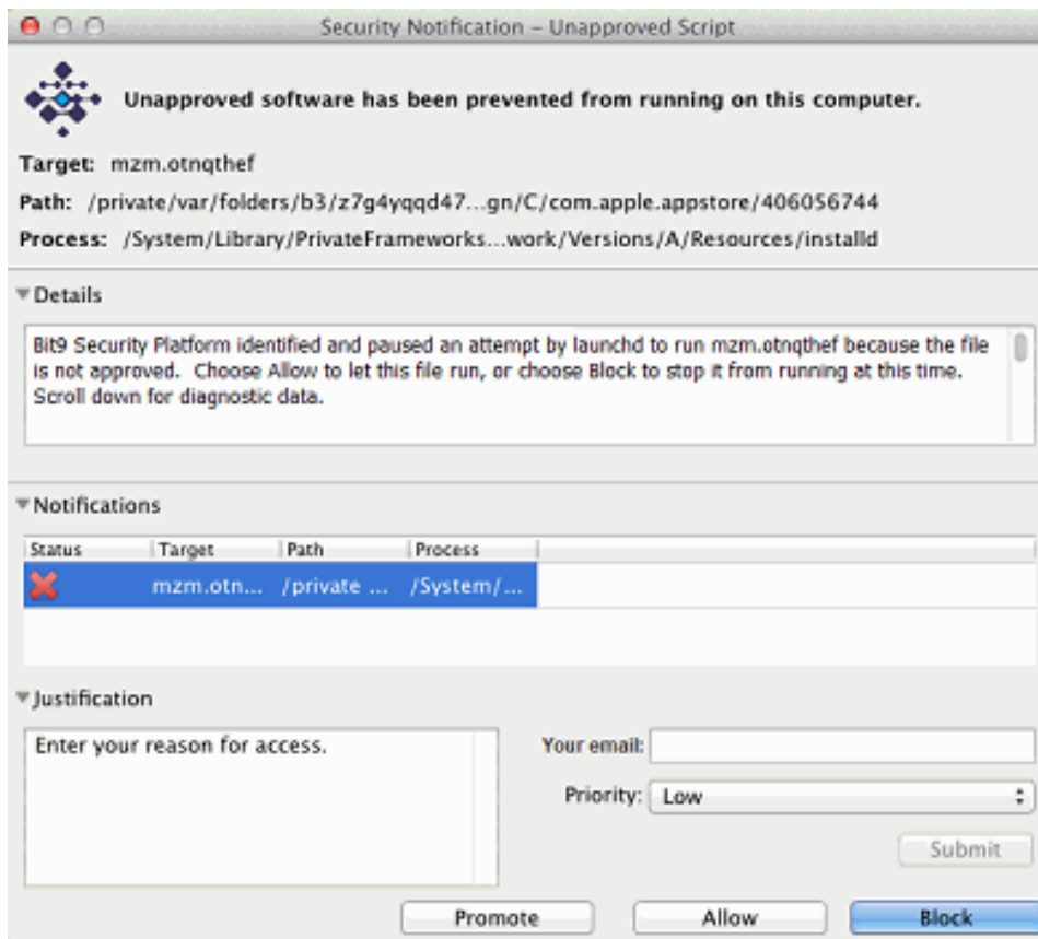
Prompt Notifier on Mac -- with Justification panel
