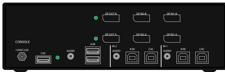
Figure 4-2: KVS4-2002VX Rear panel
