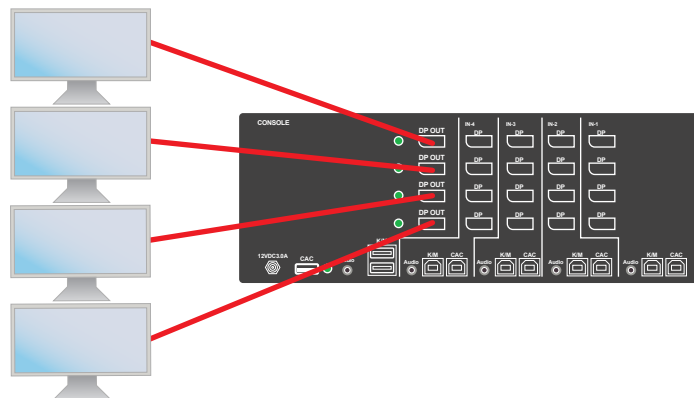
Figure 7-2: KVS4-4004VX
