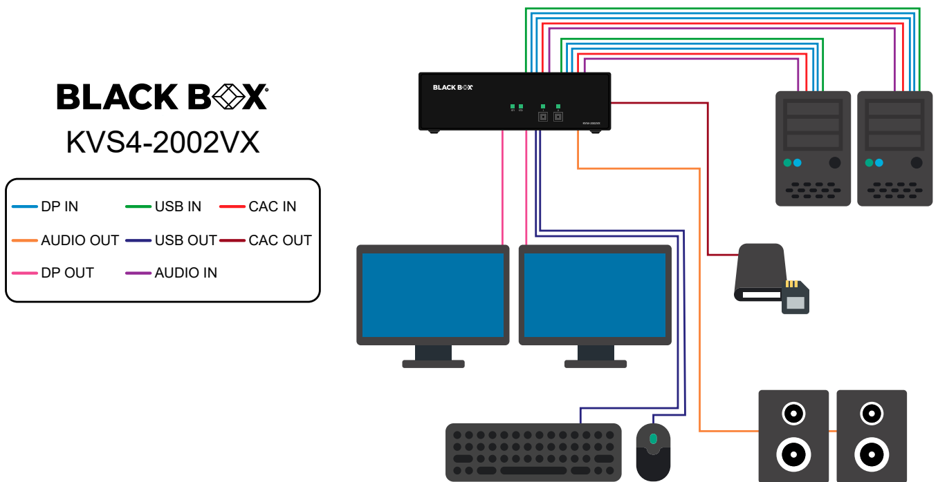
Figure 8-2: KVS4-2002VX
