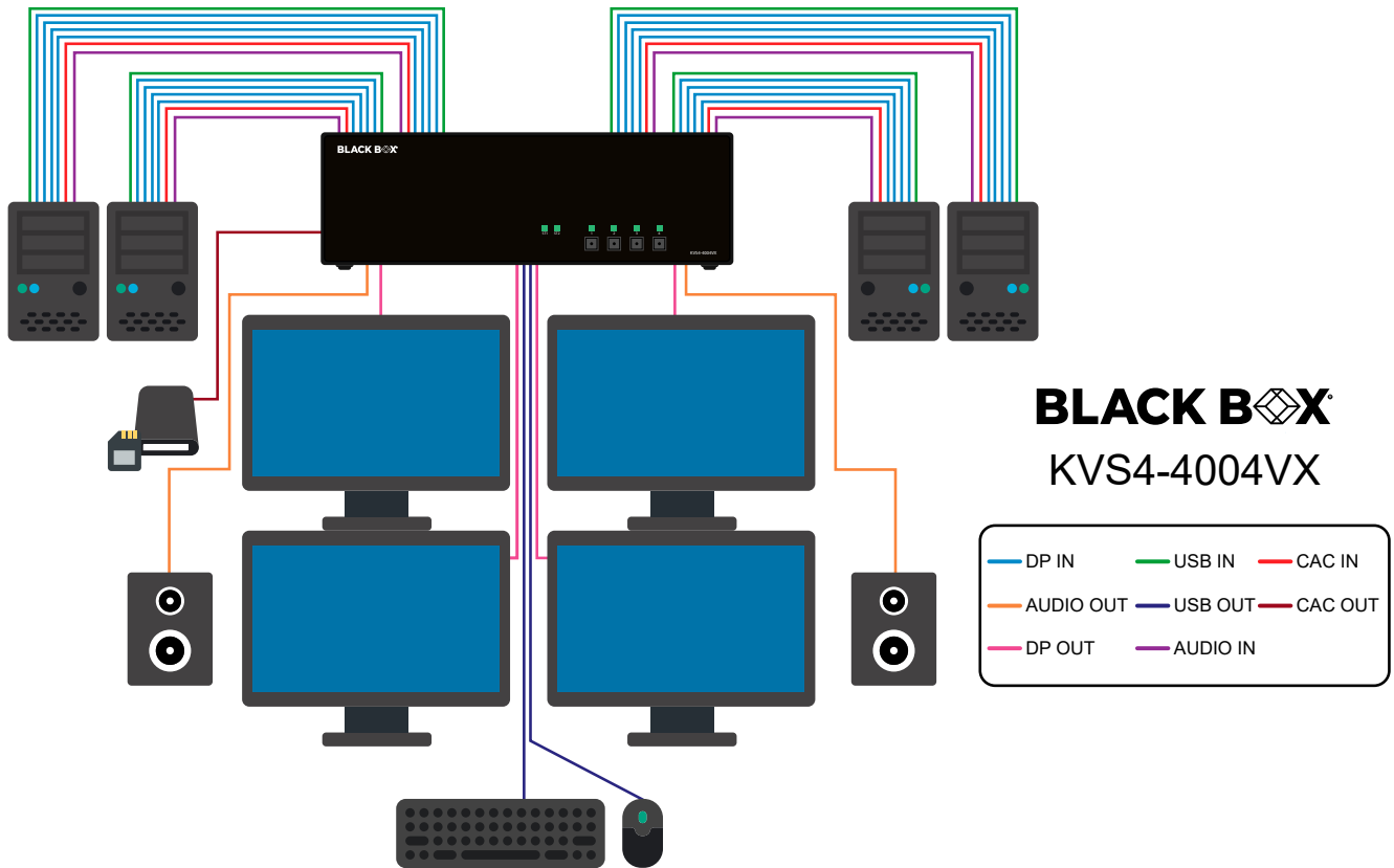
Figure 8-1: KVS4-4004VX
