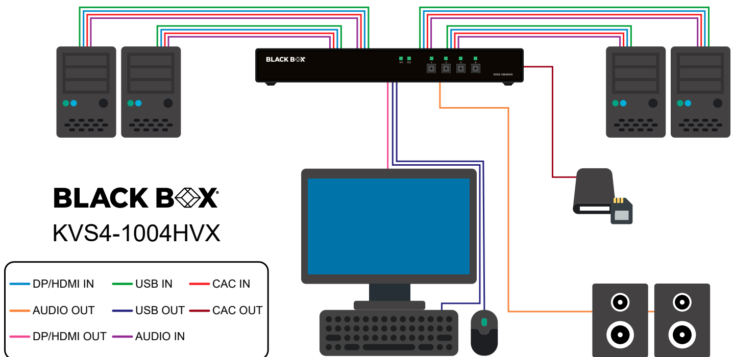
Figure 6-1: KVS4-1004HVX
