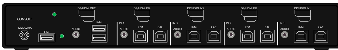
Figure 4-2: KVS4-1004HVX Rear panel
