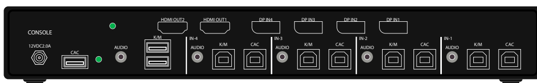
Figure 4-2: KVS4-1004VMX Rear panel
