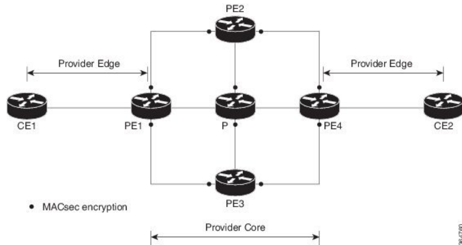
Figure 8: MACsec on Physical Interfaces in an MPLS Core Network
