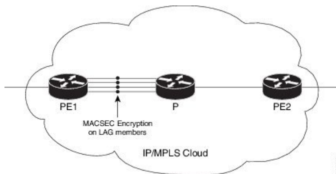
Figure 9: MACsec on a Link Bundle in an MPLS Core Network
