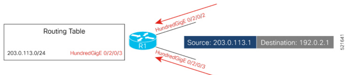
Figure 10: uRPF in Loose Mode
