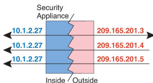
Figure 60: One-to-Many Static NAT
