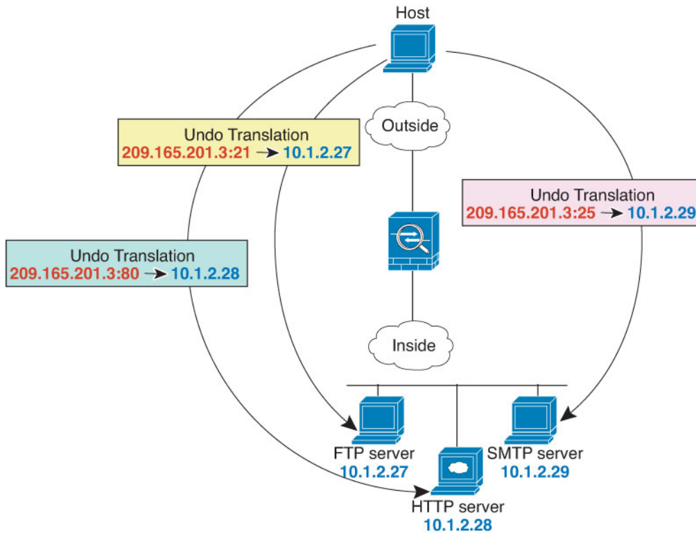
Figure 68: Static NAT-with-Port-Translation
