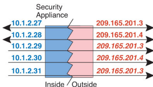
Figure 63: Many-to-Few Static NAT
