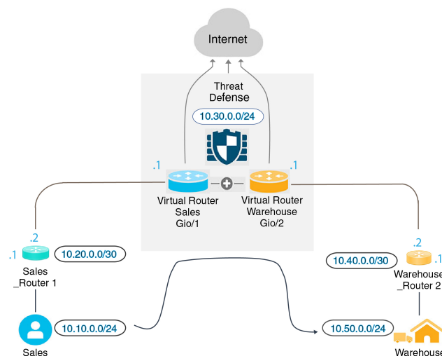
Figure 41: Interconnecting Two Virtual Routers - An Example
