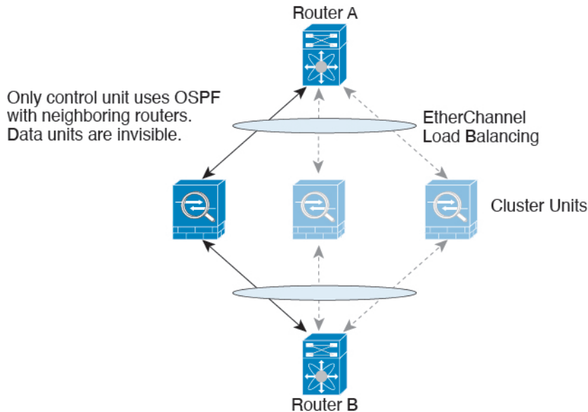
Figure 39: Dynamic Routing
