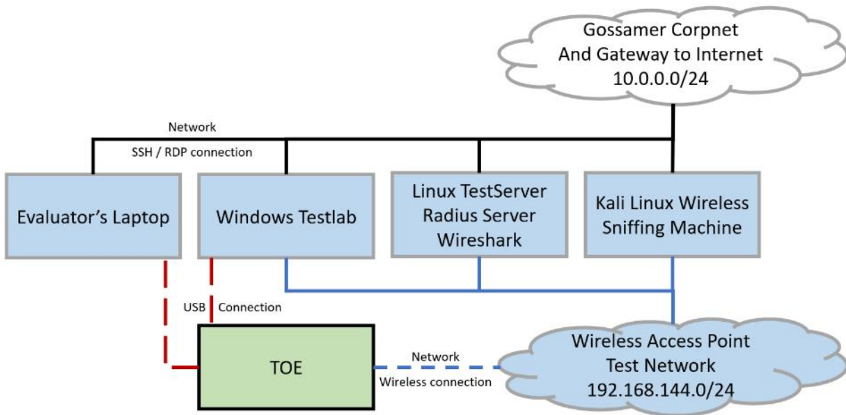
Figure 1 Test Setup
