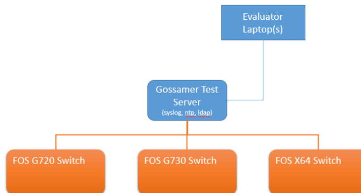
Figure 1 Test Setup
