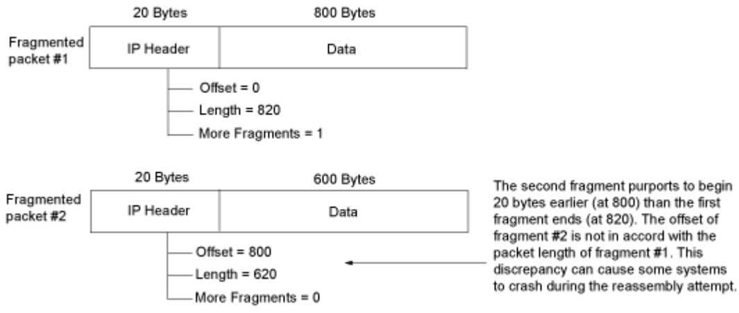
Figure 12: Fragment Discrepancy
