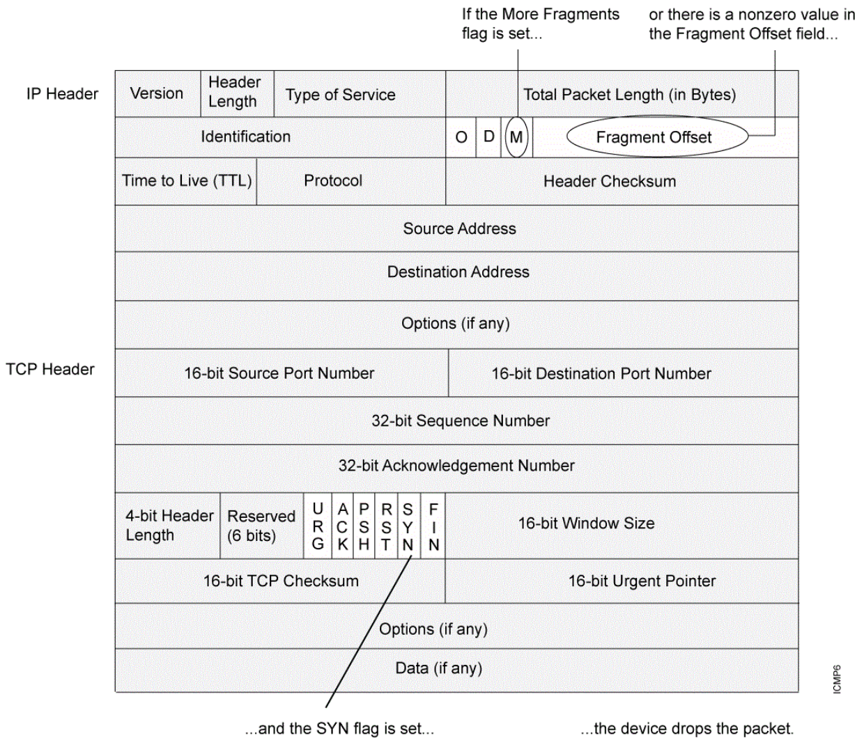
Figure 16: SYN Fragments
