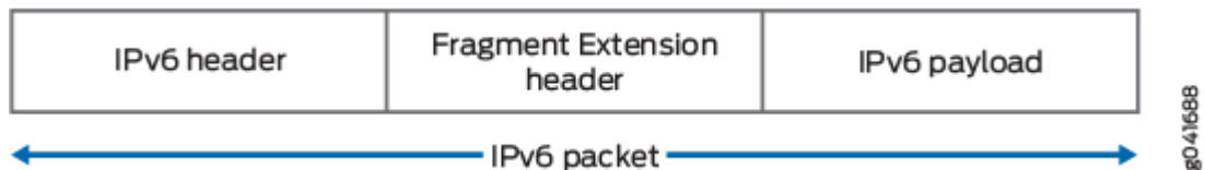
Figure 18: IPv6 Packet
