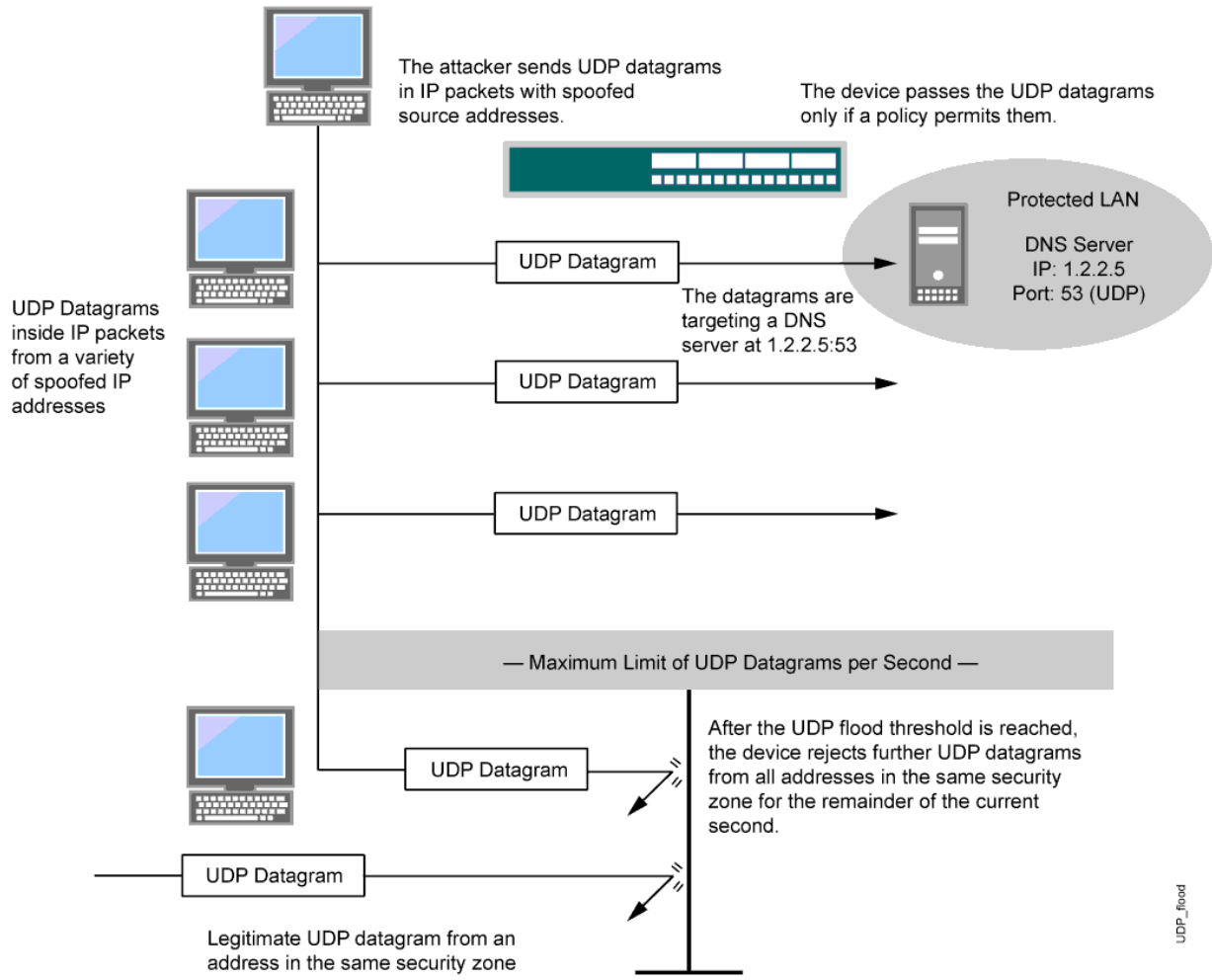
Figure 8: UDP Flooding
