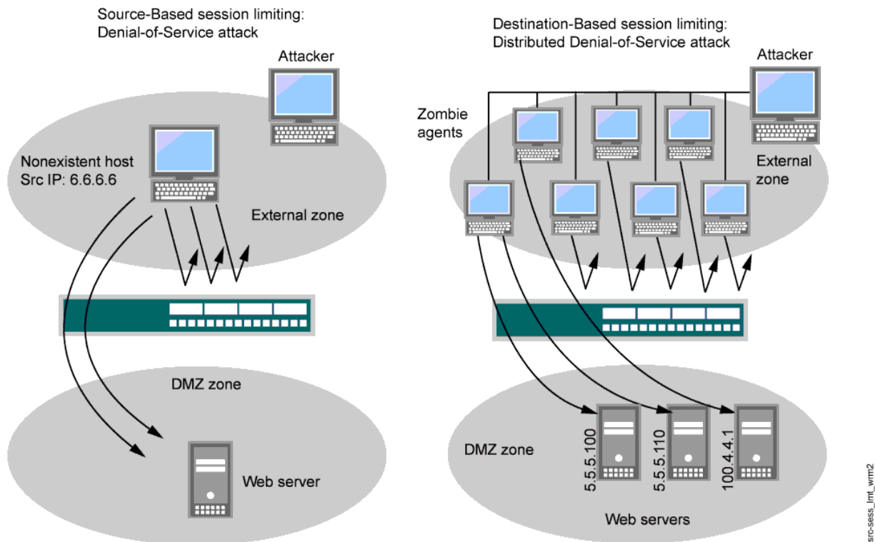
Figure 2: Distributed DOS Attack
