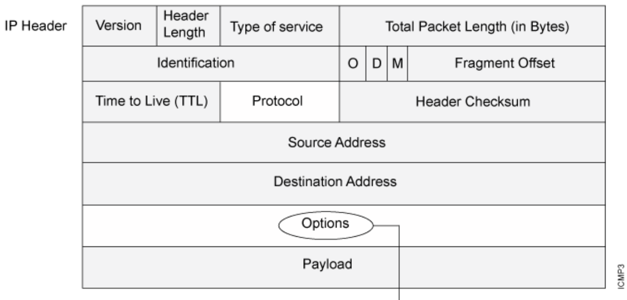
Figure 20: Incorrectly Formatted IP Options
