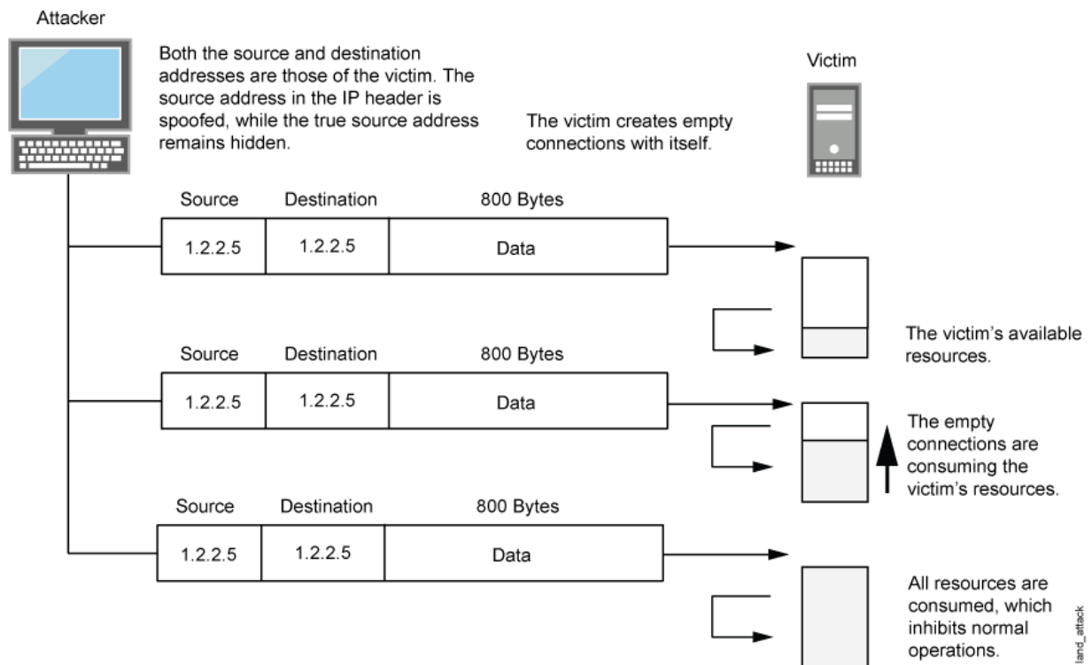
Figure 9: Land Attack
