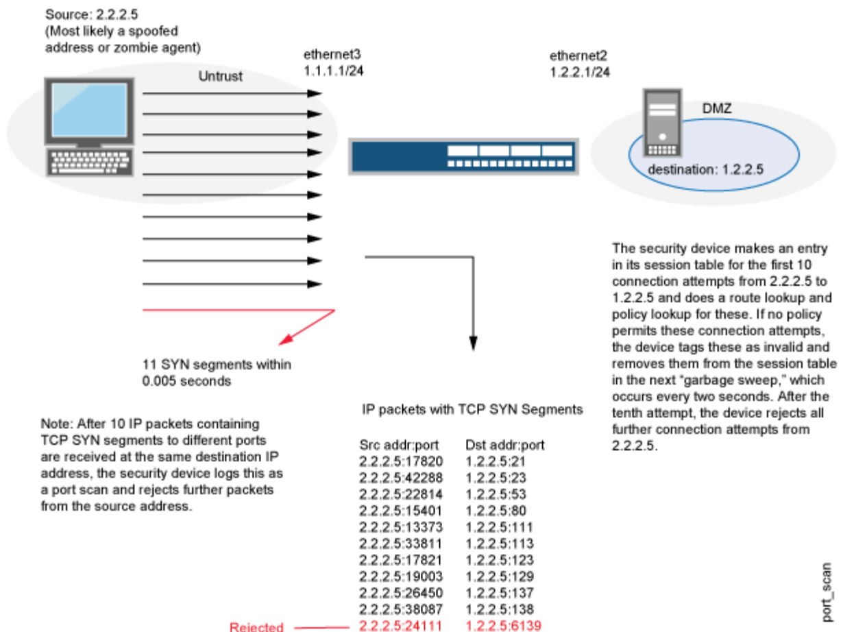
Figure 24: Port Scan
