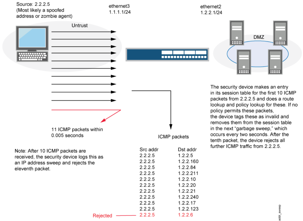
Figure 23: Address Sweep
