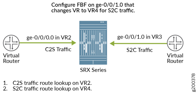
Figure 30: Reverse Route Enabled with FBF
