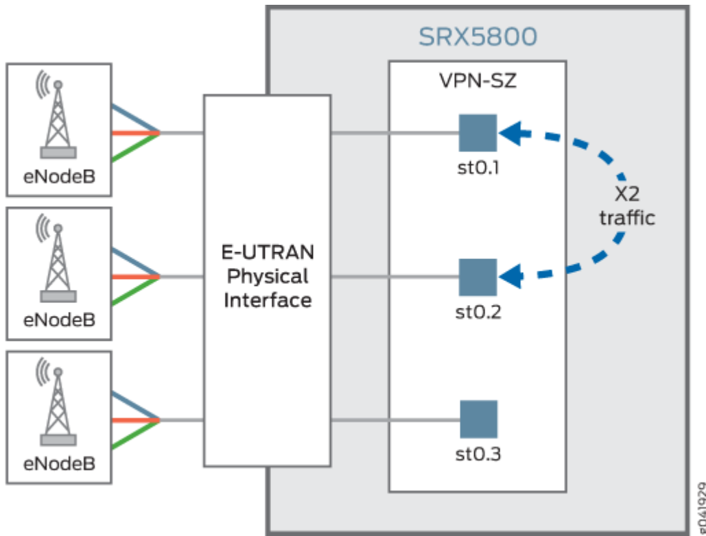
Figure 21: SRX Series Firewall in an LTE Mobile Network
