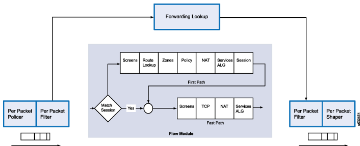
Figure 25: Traffic Flow with Selective Stateless Packet-Based Services
