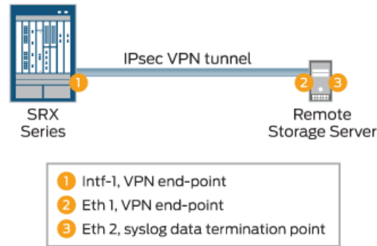
Figure 1: IPsec VPN Tunnel
